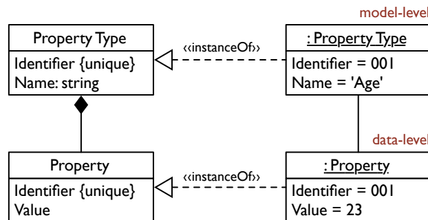
Figure 3.4: A class diagram of the PROPERTY pattern.
