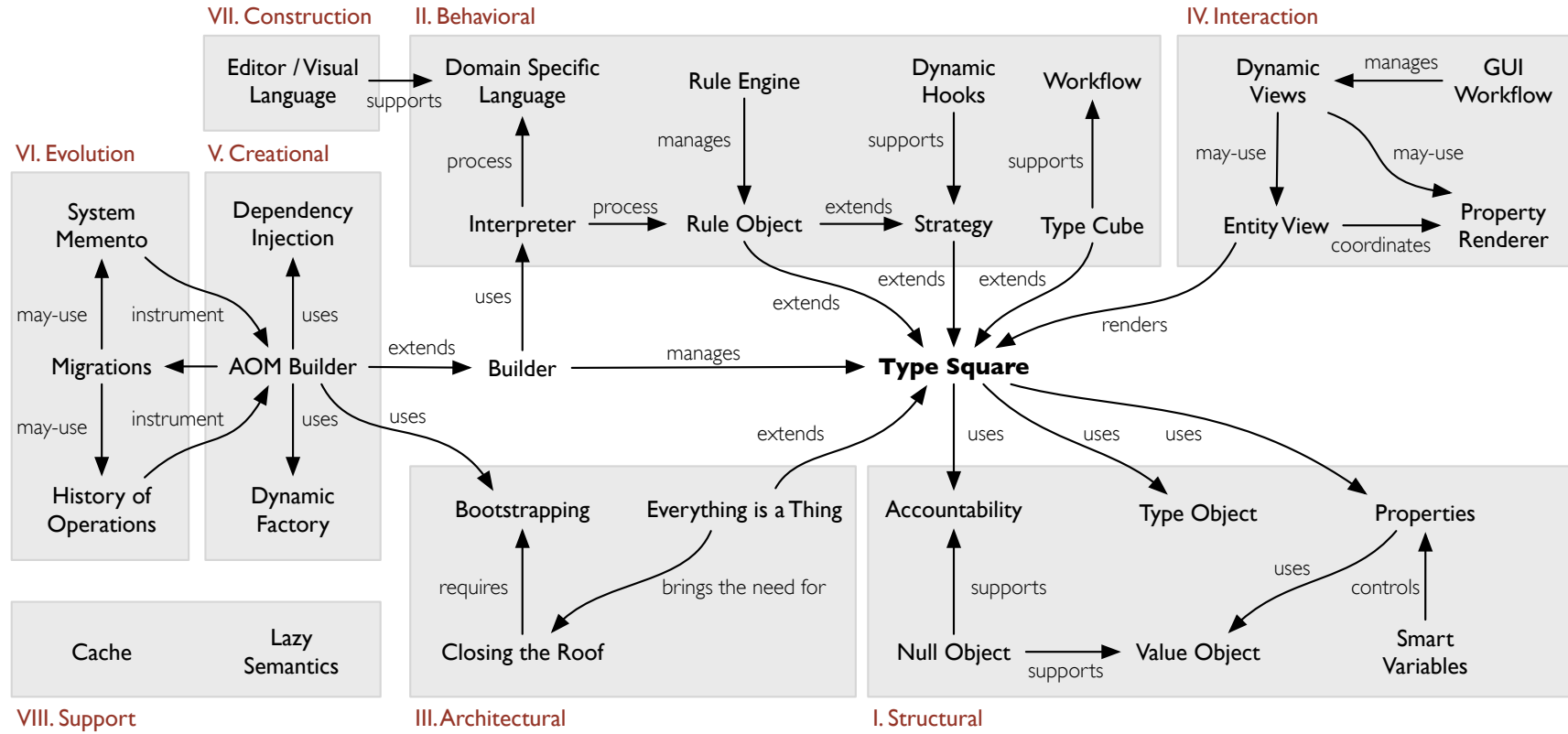
Figure 5.12: Proposed evolution of the pattern language for Adaptive Object-Models.
